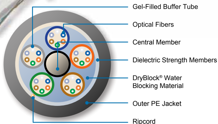
PowerGuide TTH Cable Cross-Section
